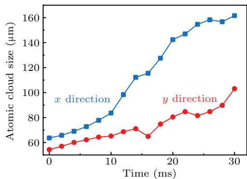
Fig. 9. Experimental observation of the expansion of BEC in accordion lattice. The measured atomic cloud sizes along the x and y axes when turning off the 1064 \text{ nm} single beam trap and keeping the accordion lattice on until the absorption imaging finished.
