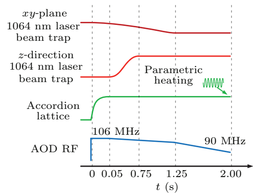
Fig. 5. Time sequence for preparing the 2D BEC. The intensities of optical dipole trap laser beams are shown by the red lines while that of the accordion lattice beams is shown by the green line. The green wiggly curve shows the amplitude modulation of the accordion lattice beams to measure the trapping frequencies of the accordion lattice, also called parametric heating method.
