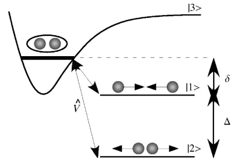
FIG. 1. The p -wave model: we consider three internal states, labeled |1\rangle , |2\rangle , and |3\rangle . States |1\rangle and |2\rangle are two open channels corresponding, respectively, to the incoming and decay channels. The released energy in an inelastic collision bringing an atom initially in |1\rangle to |2\rangle is denoted \Delta . State |3\rangle is a closed channel that possesses a p -wave bound state of energy \delta nearly resonant with state |1\rangle . Finally, we assume that these three channels interact through a potential \hat{V} acting only on the internal states and coupling the two open channels to the closed channel.
